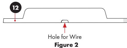
Base 12 (Bottom View)
