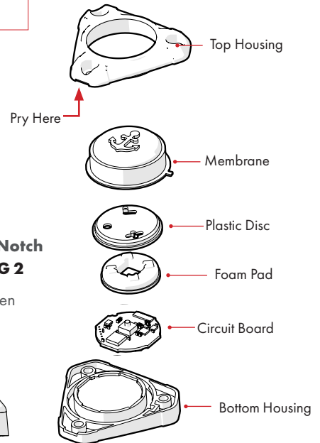
Exploded View
